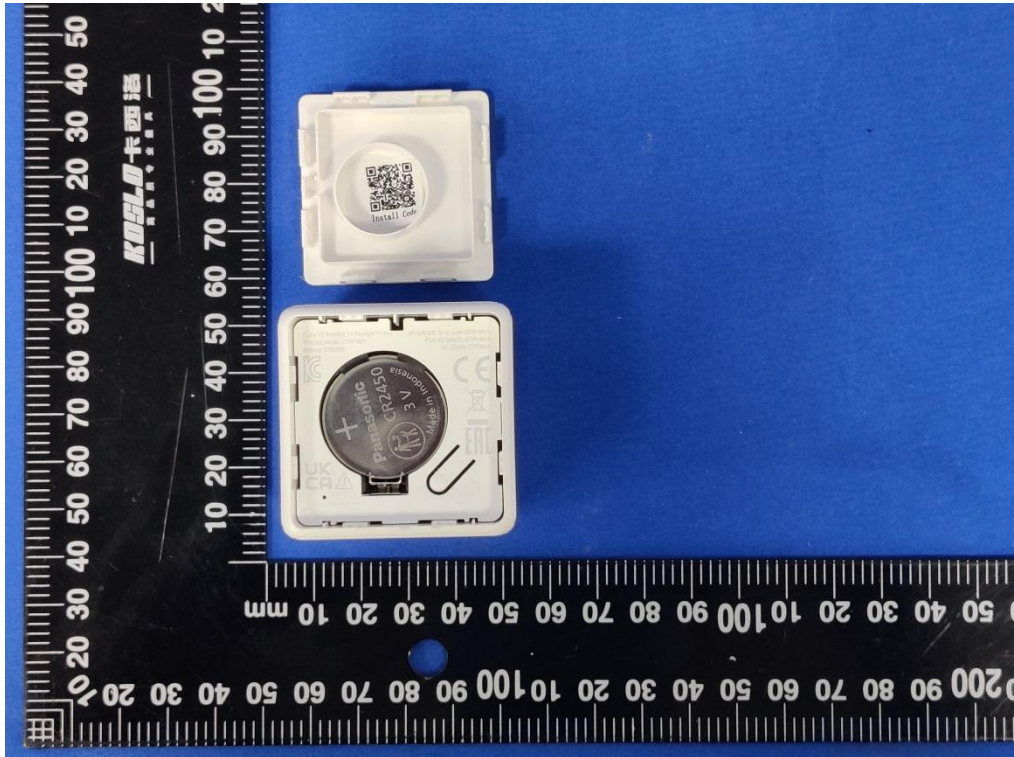
Fig.3 Internal view
