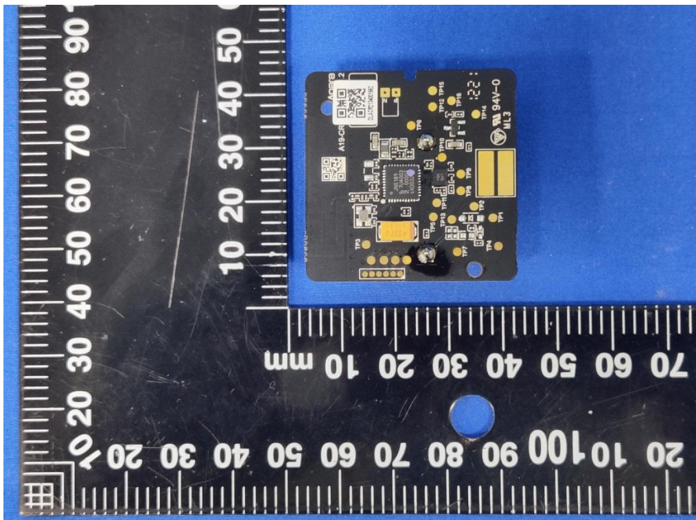
Fig.6 PCB view
