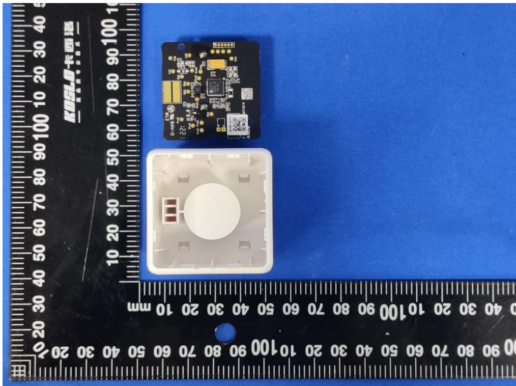
Fig.5 Internal view
