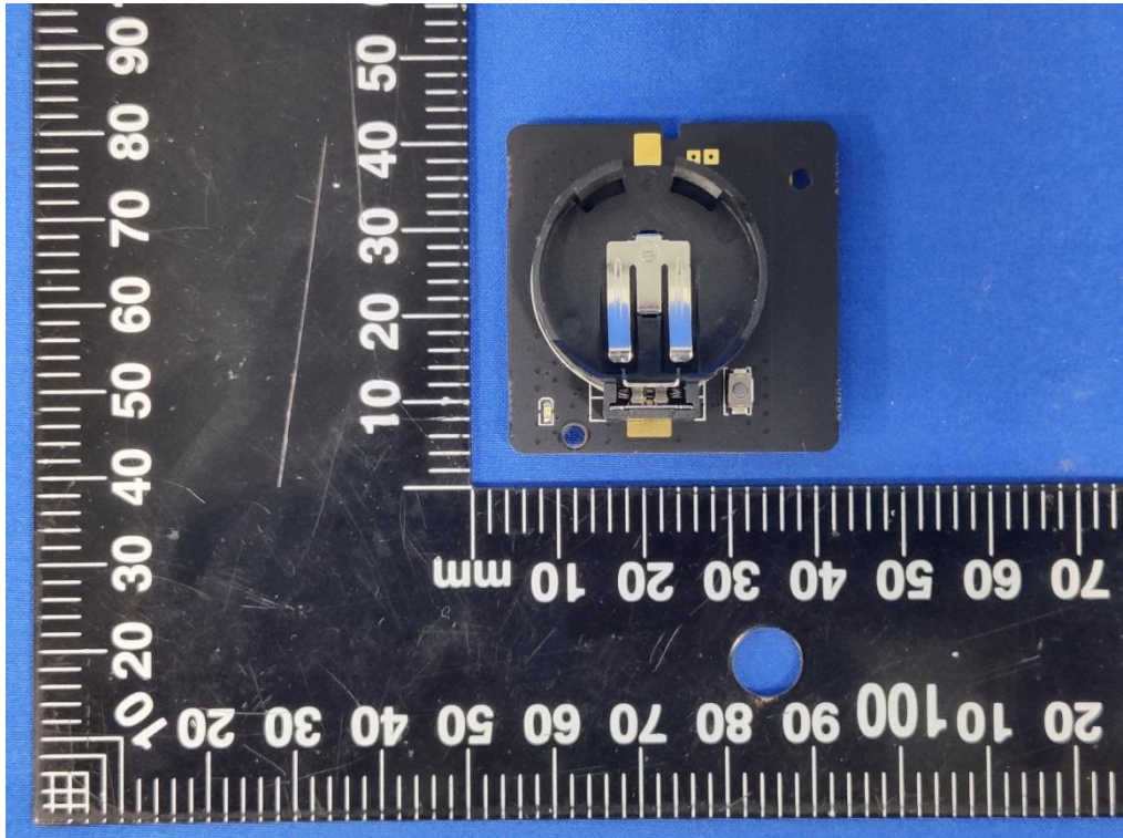
Fig.7 Internal view
