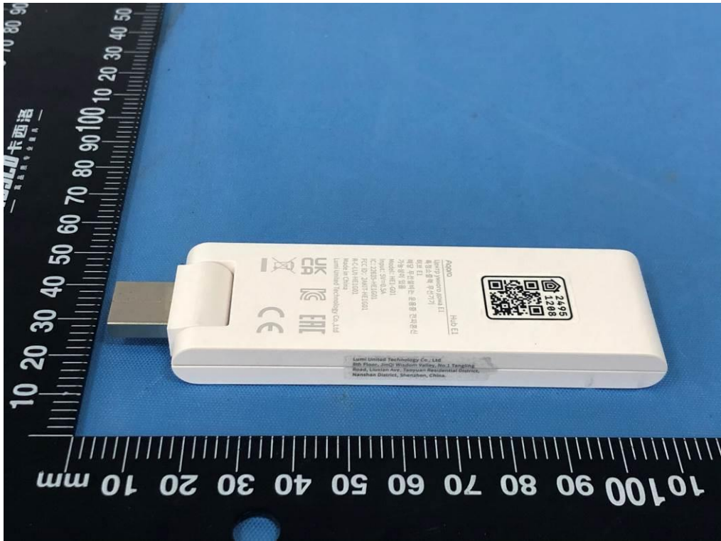
Fig.5 Side view
