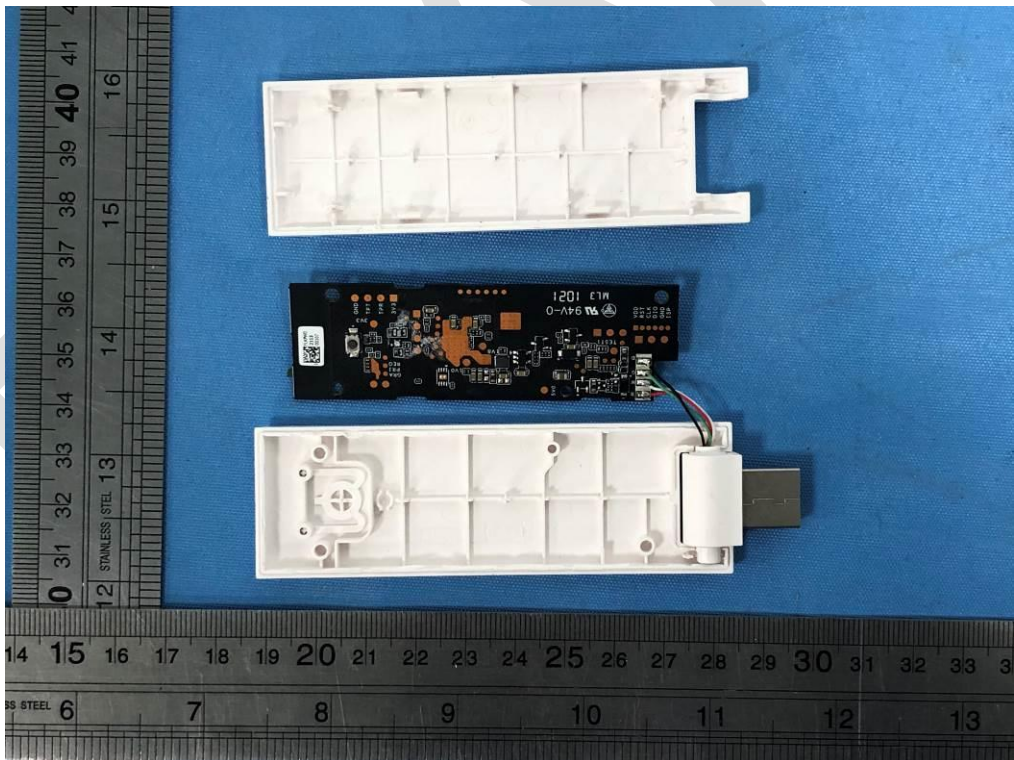
Fig.6 Internal view
