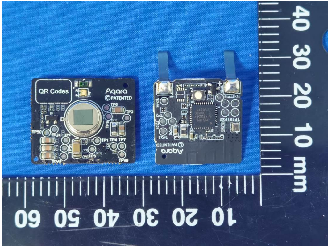
Fig.9 PCB view
