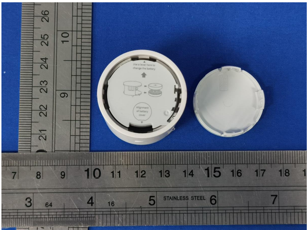
Fig.4 Internal view
