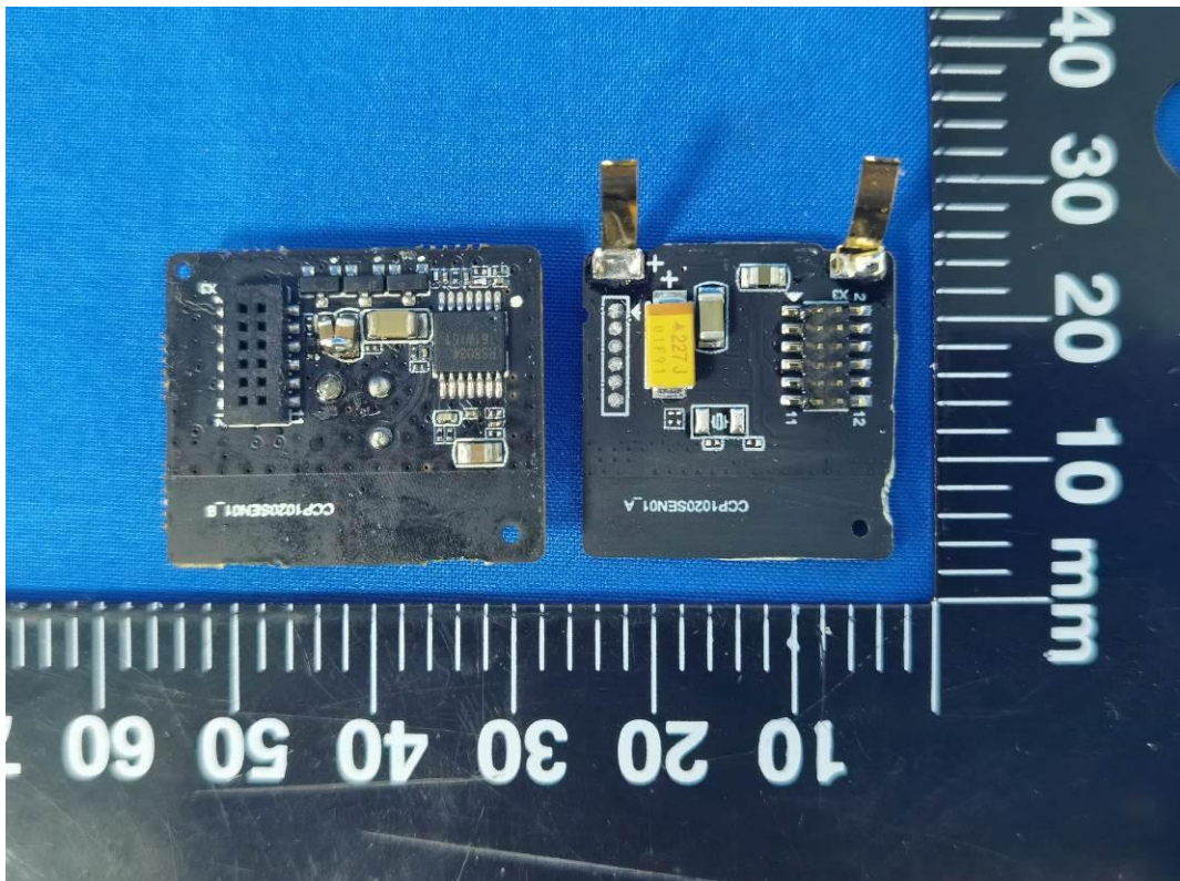
Fig.8 PCB view
