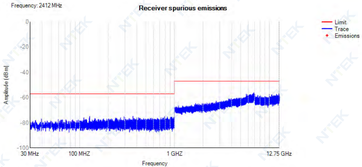
Rx. Spurious NVNT 802.11b 2412MHz
