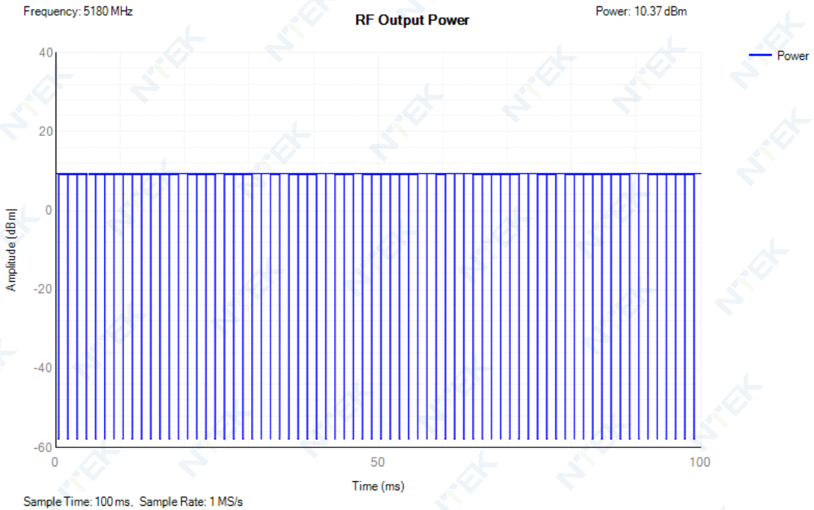
Power NVNT 802.11a 5180MHz
