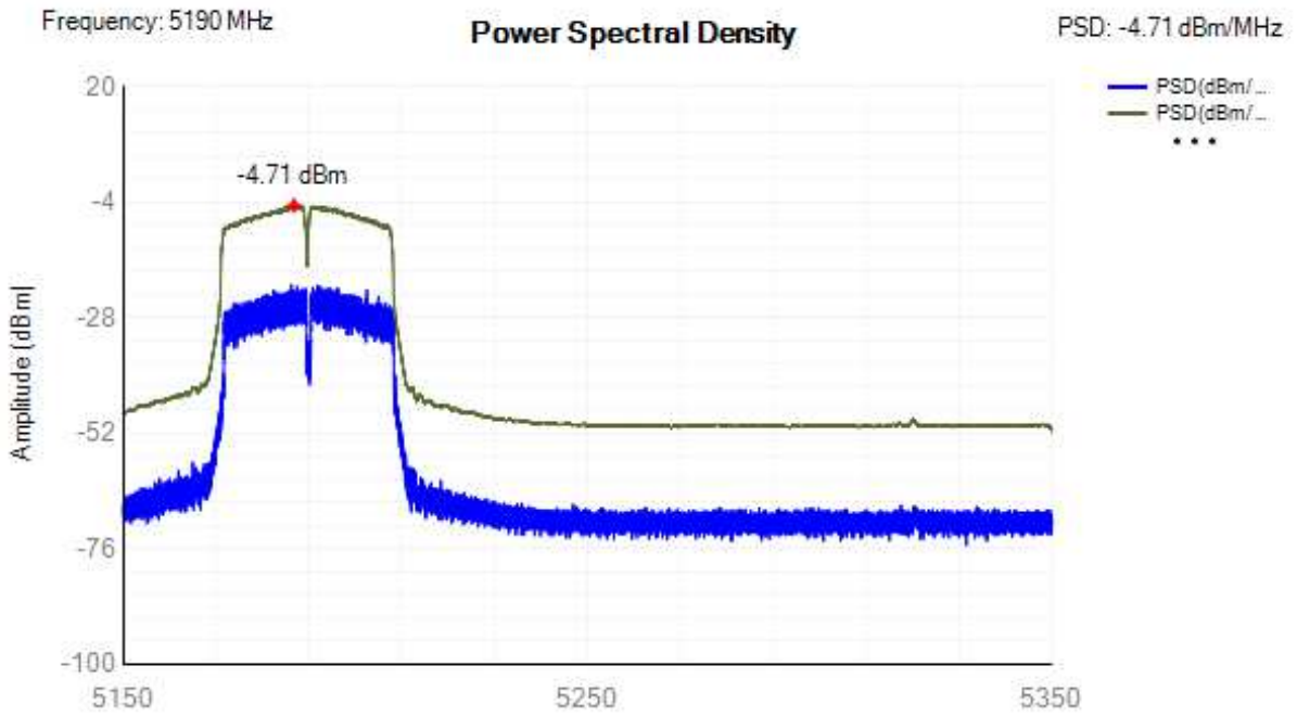
PSD NVNT ac40 5190MHz Ant1
