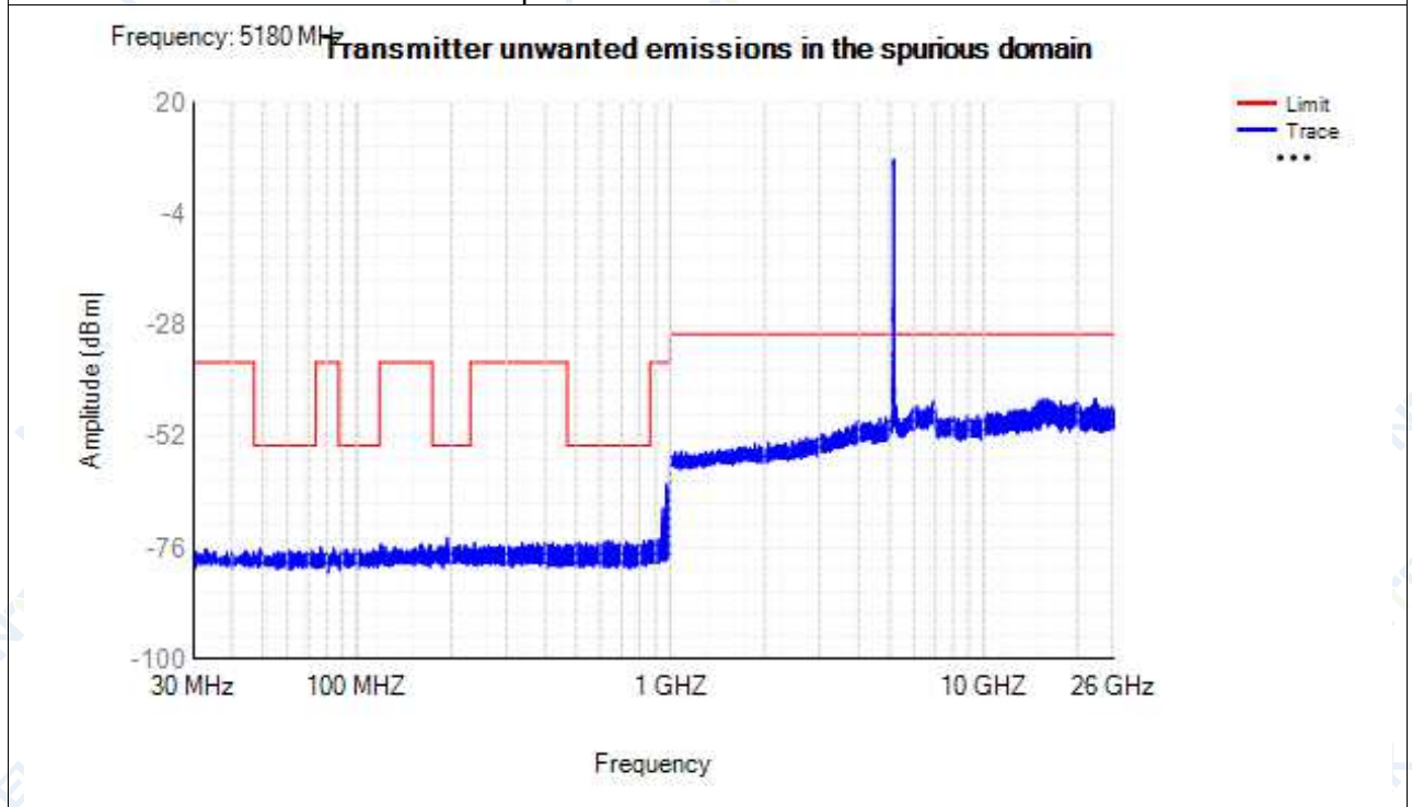
Tx. Spurious NVNT a 5180MHz Ant1
