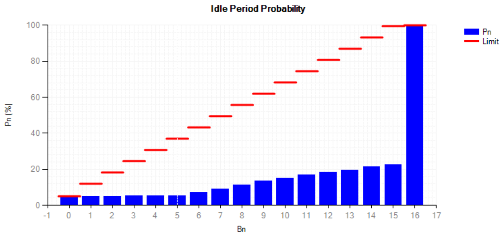
Idle Period Probability NVNT 802.11n(HT40) 5190MHz
