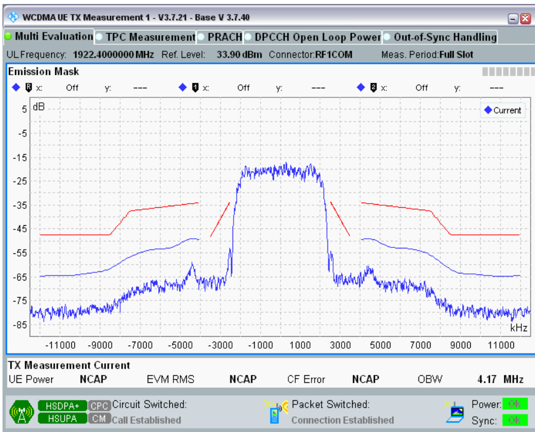
HSUPA Band1 Channel=9612 Subtest1
