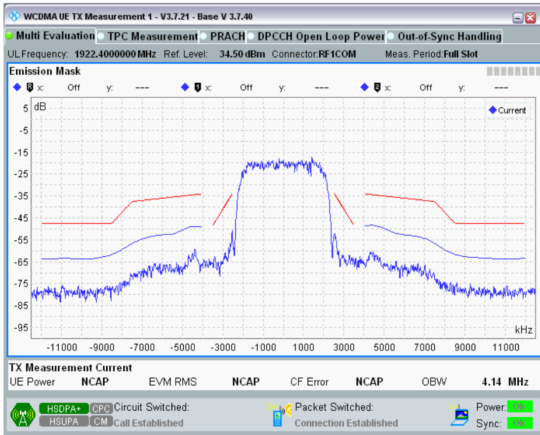
HSDPA Band1 Channel=9612 Subtest1
