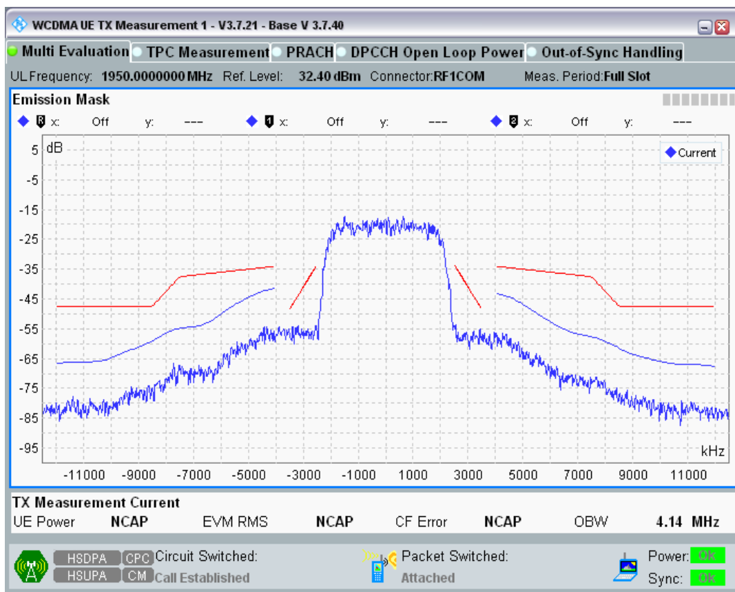
WCDMA Band1 Channel=9612
