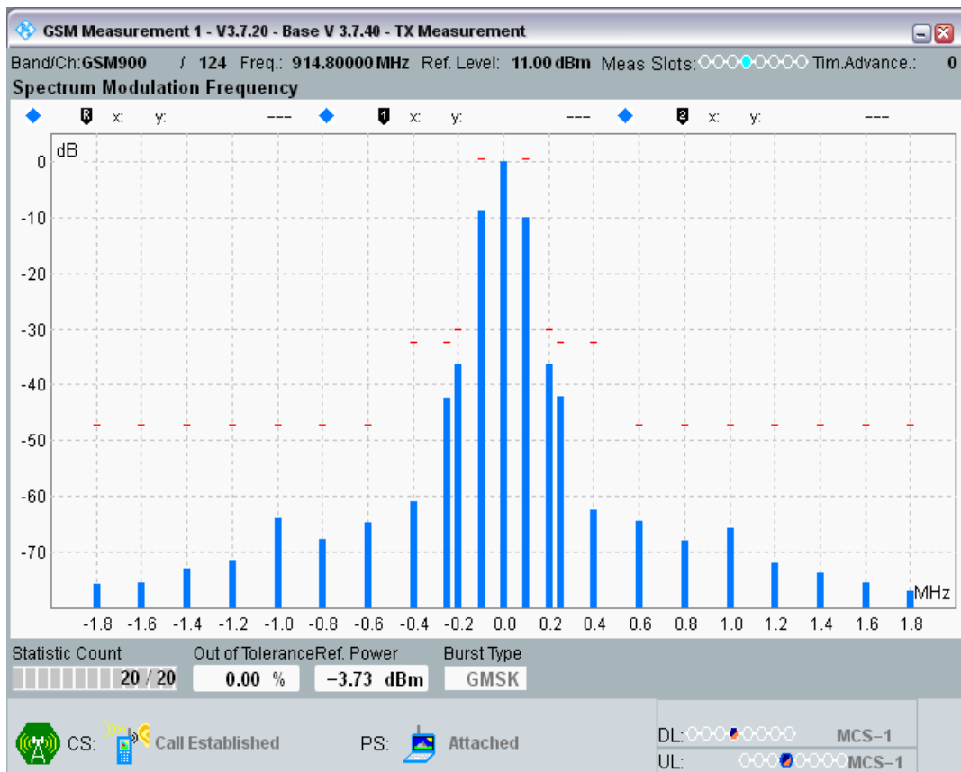
Clause 4.2.6 Transmitter-Switching Spectrum
