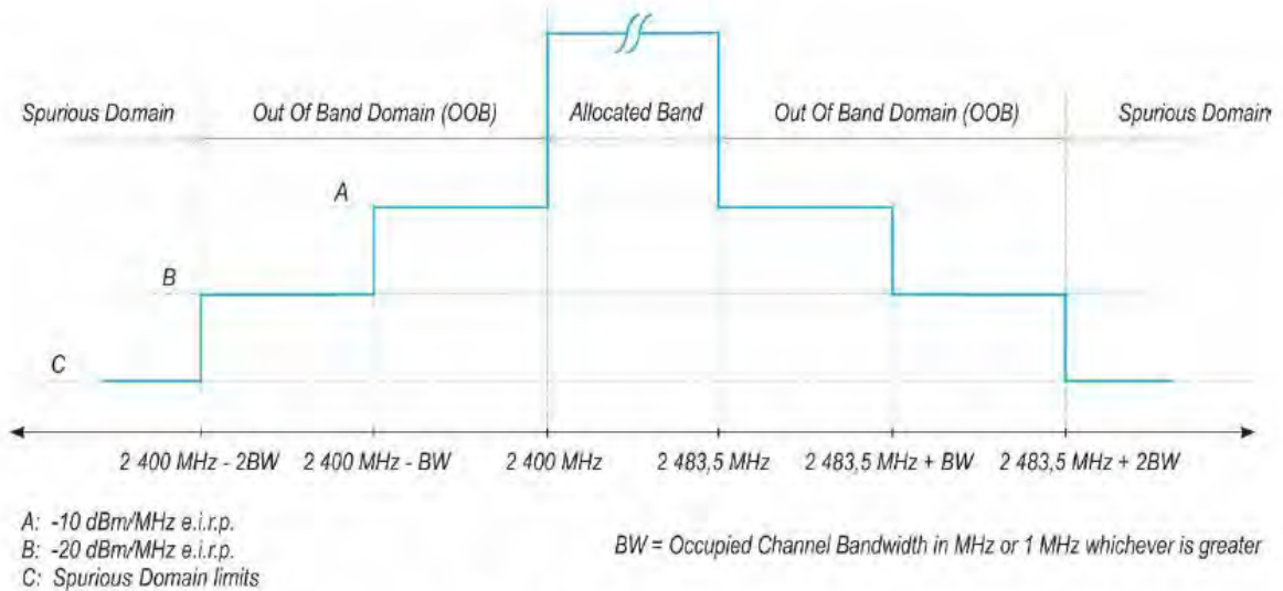
Figure 1: Transmit mask
