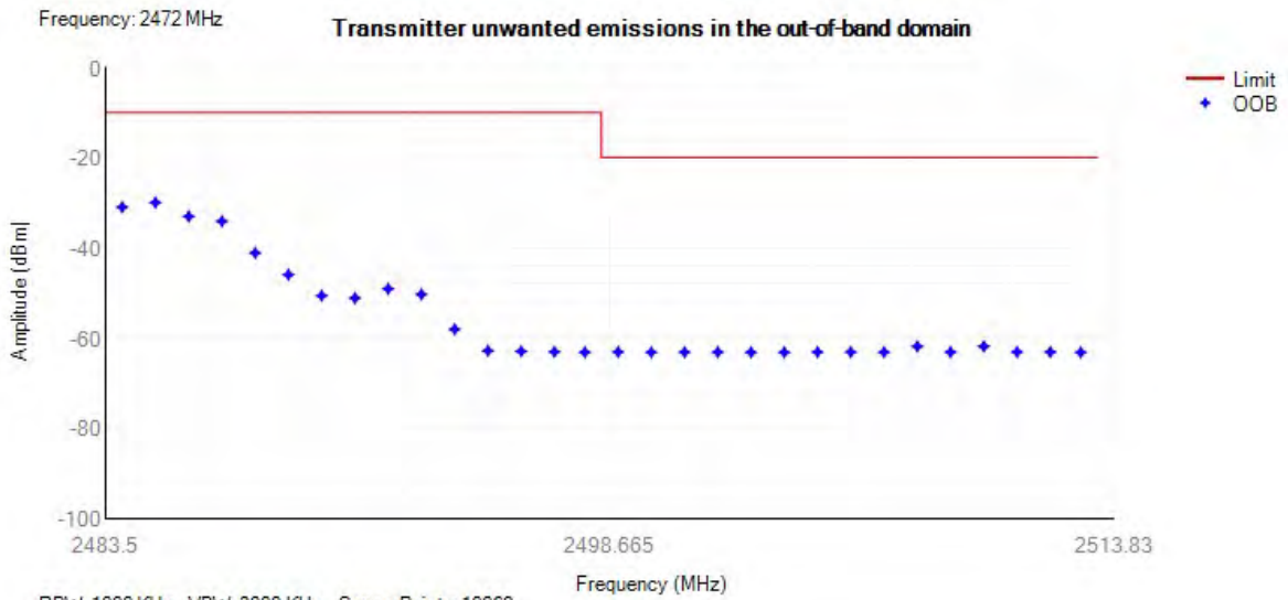
Tx. Emissions OOB NVNT 802.11g 2412MHz
