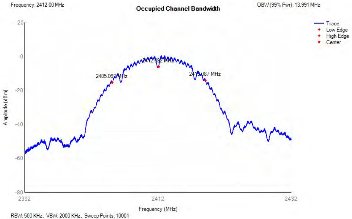
OBW NVNT 802.11b 2412MHz
