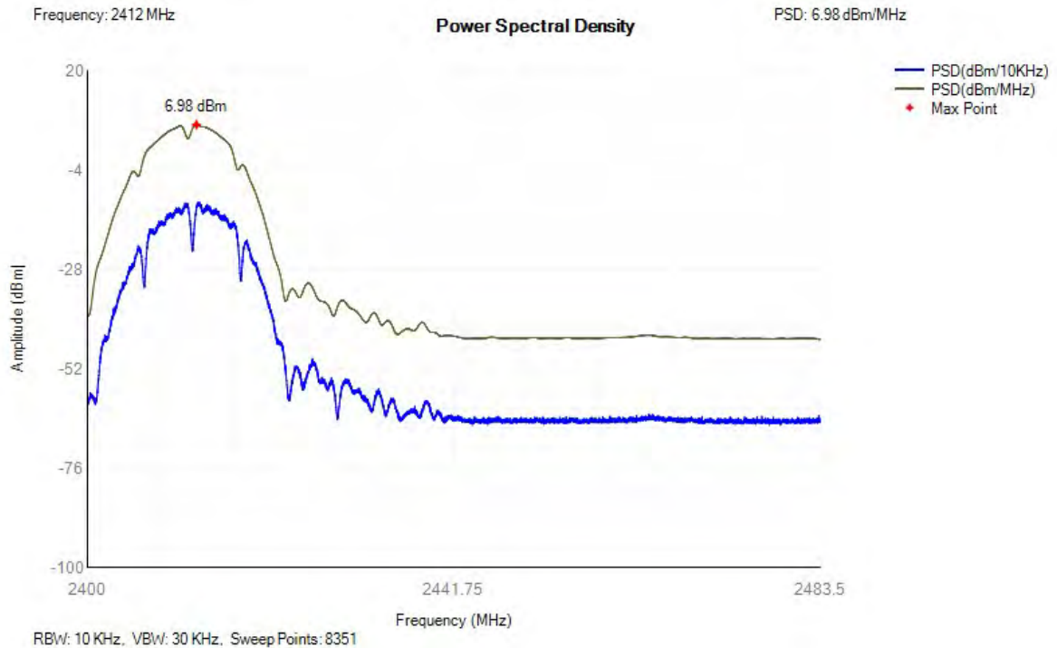
PSD NVNT 802.11b 2412MHz
