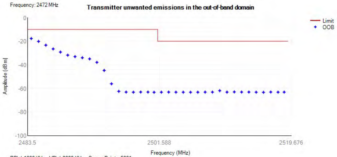
Tx. Emissions OOB NVNT 802.11g 2472MHz
