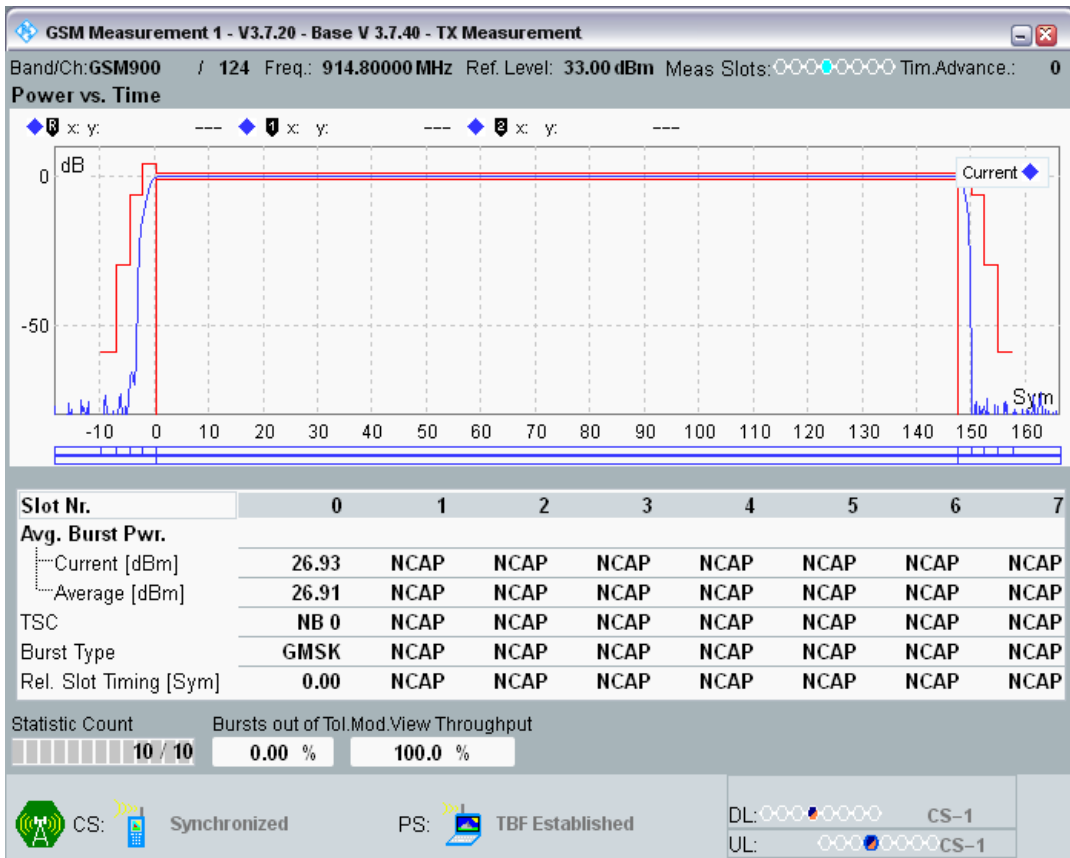
GPRS900 Channel=124 Gamma=7;7;7;7
