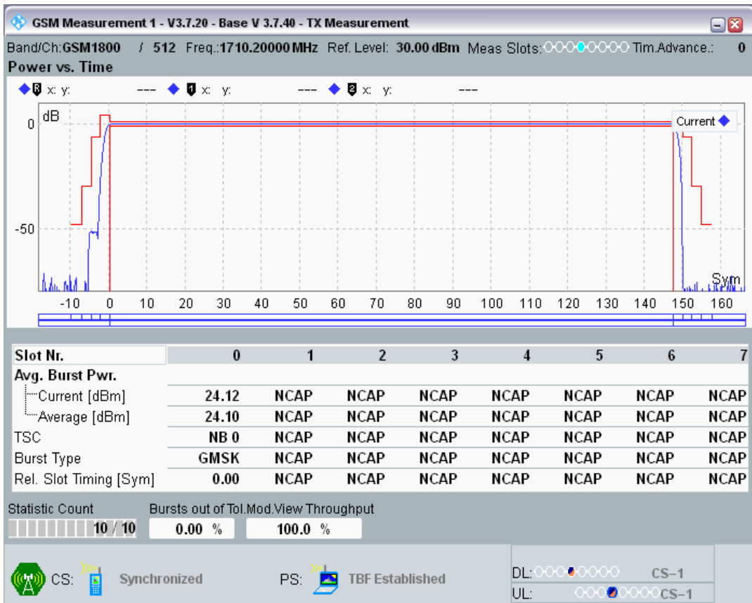
GPRS1800 Channel=512 Gamma=7;7;7
