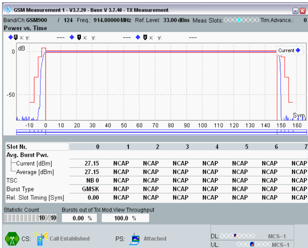
GSM900 Channel=124 PCL=10
