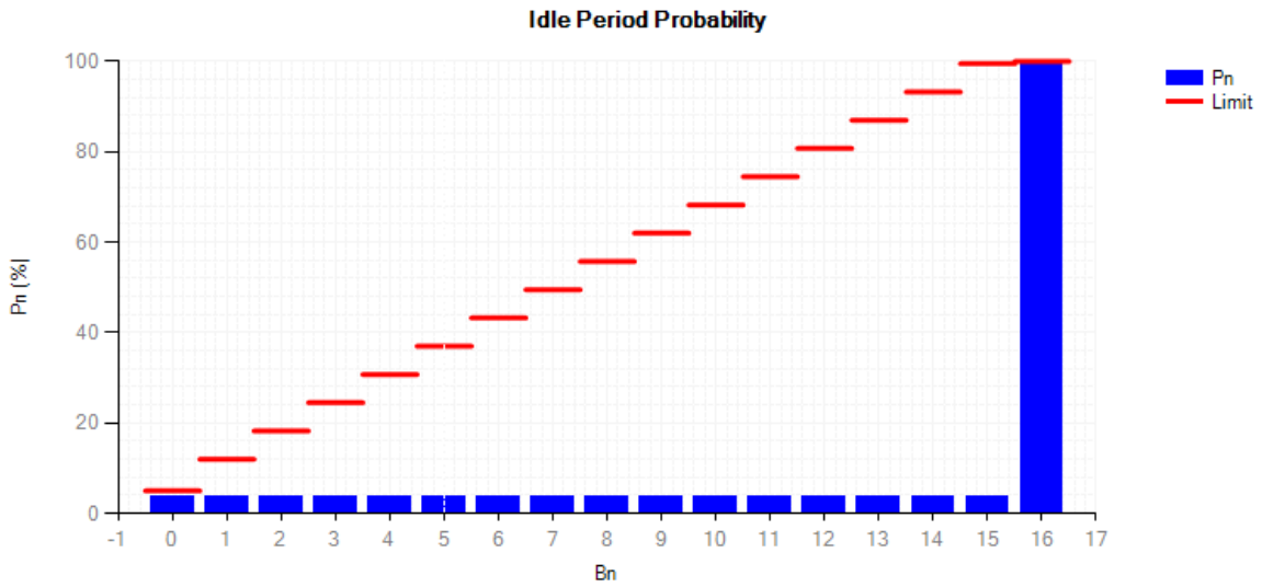
Idle Period Probability NVNT 802.11a 5320MHz
