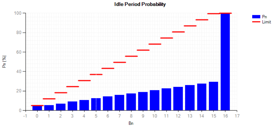
Idle Period Probability NVNT 802.11n(HT40) 5310MHz
