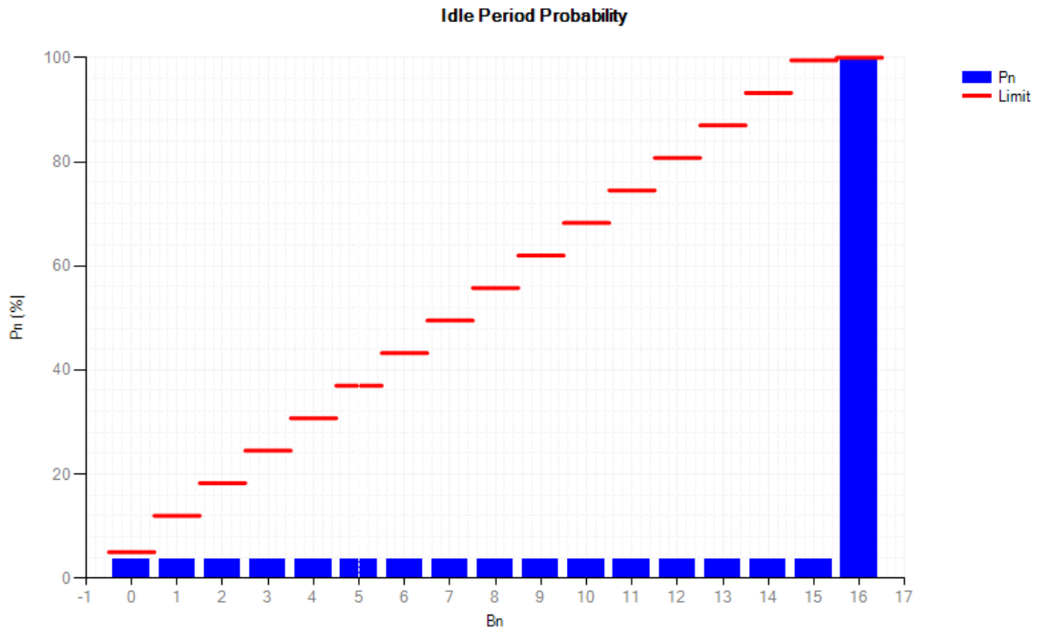
Idle Period Probability NVNT 802.11ac80 5530MHz
