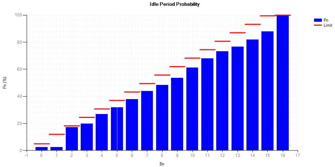
Idle Period Probability NVNT 802.11a 5320MHz
