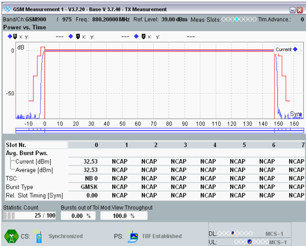
GPRS900 Channel=975 Gamma=4;4;4;4
