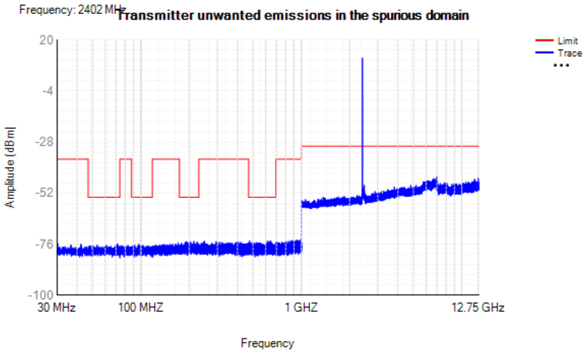
Tx. Spurious NVNT 3-DH5 2402MHz Ant1
