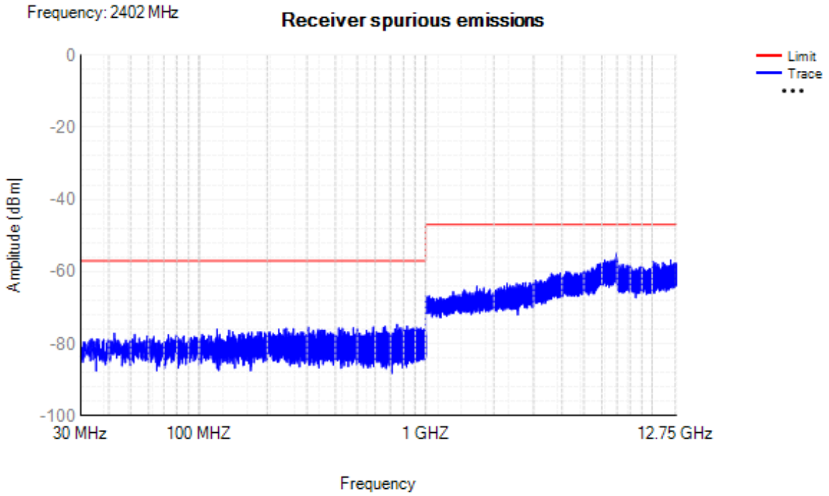
Rx. Spurious NVNT 3-DH5 2402MHz Ant1
