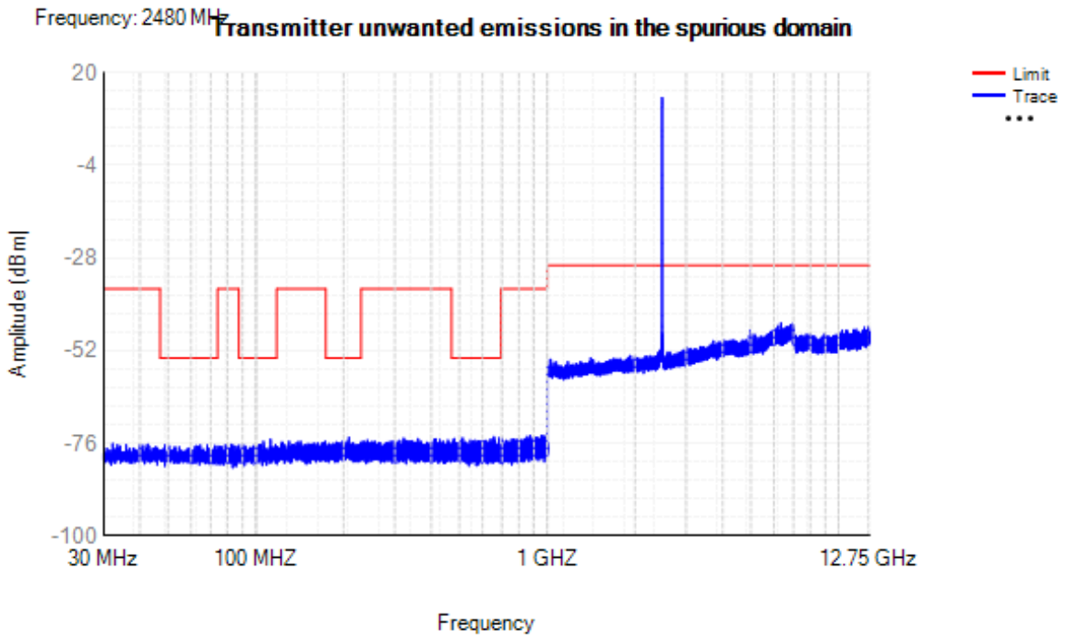
Tx. Spurious NVNT 1-DH5 2480MHz Ant1
