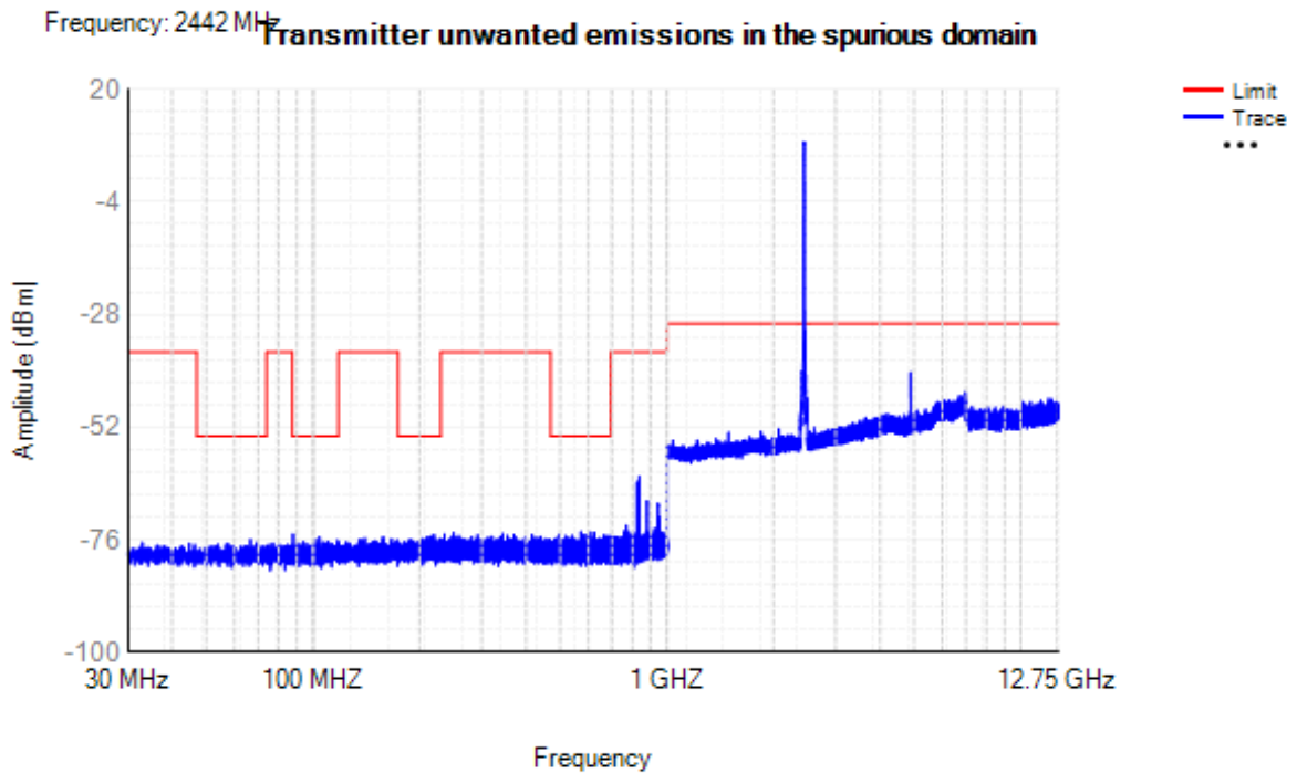
Tx. Spurious NVNT b 2442MHz Ant1
