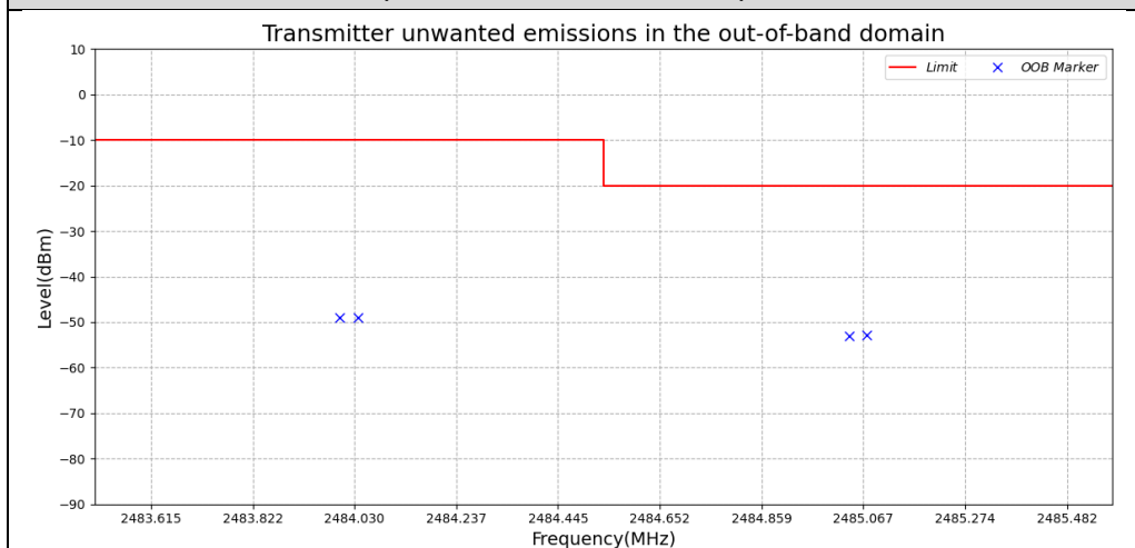
Test_Graph_LE1M_TX_2480_1Mbps_OOB_R
