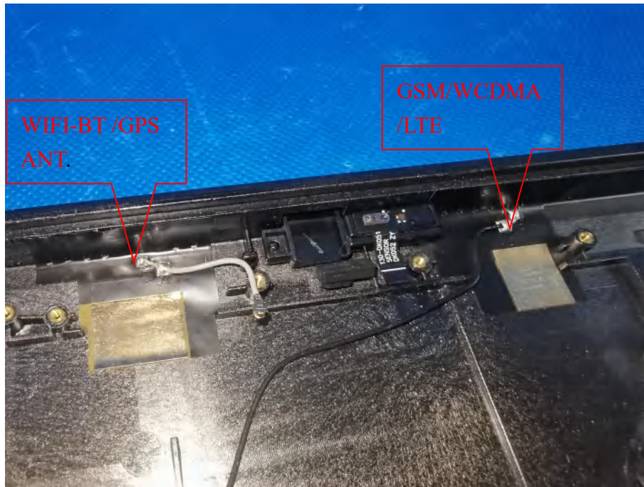
Diversity antenna
