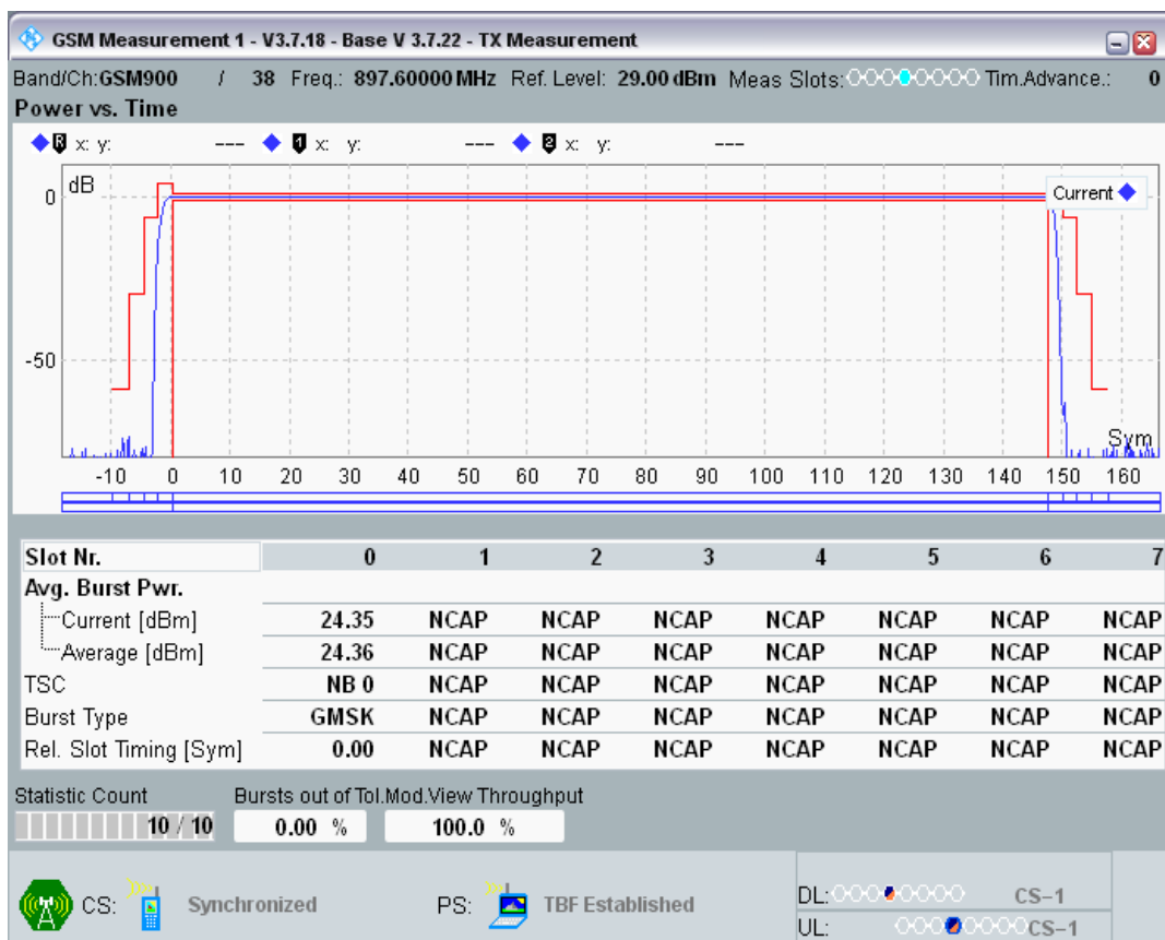
GPRS900 Channel=38 Gamma=7;7;7;7
