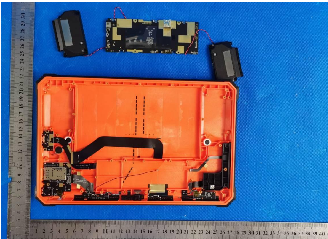
Photo 6 Internal view
