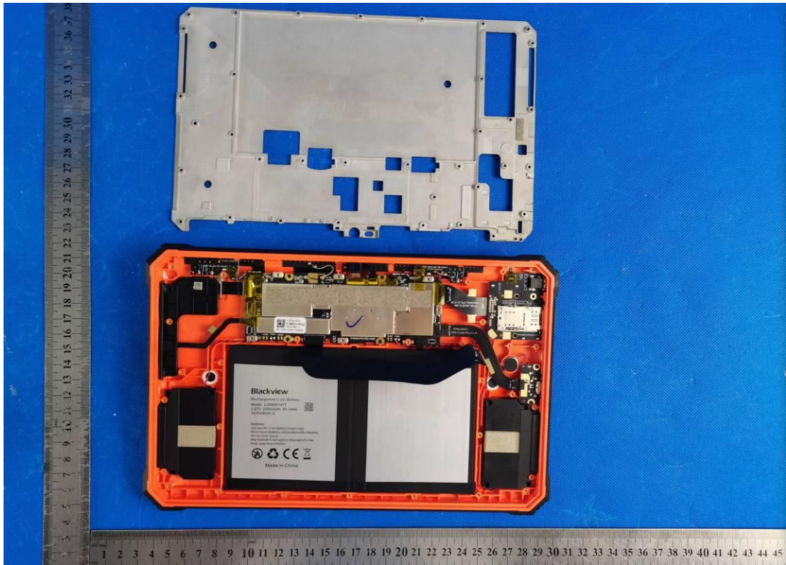
Photo 5 Internal view
