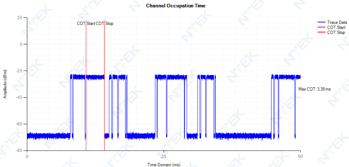
COT NVNT 802.11n(HT40) 5190MHz
