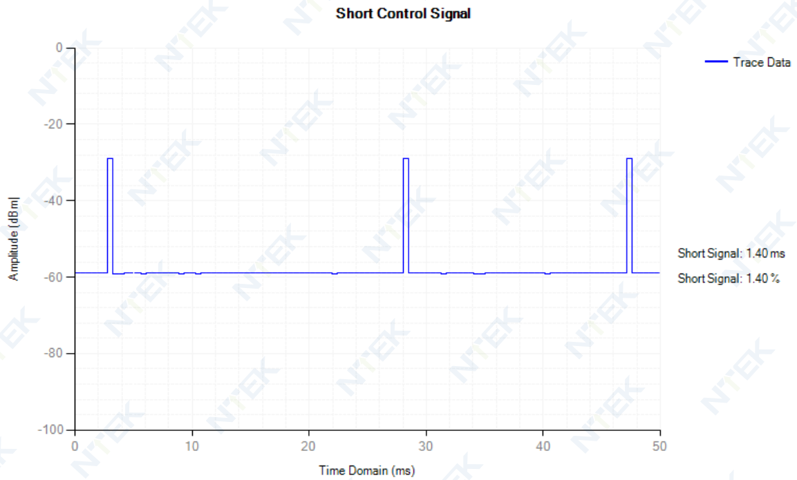
Adaptivity NVNT 802.11ac80 5210MHz LTE
