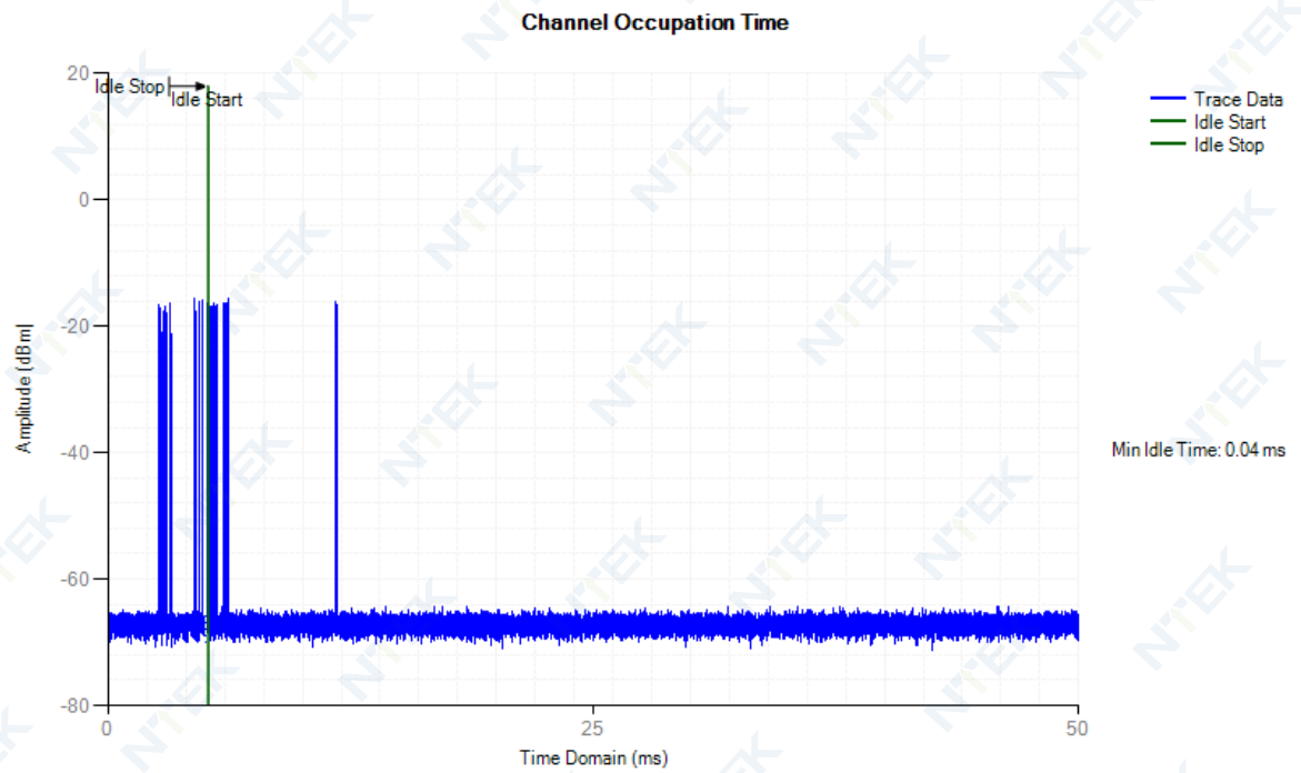
COT NVNT 802.11n(HT40) 5190MHz
