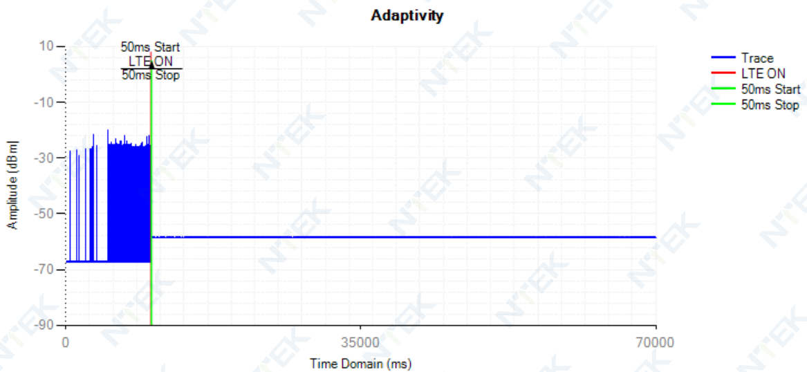
Control Signal NVNT 802.11ac80 5210MHz LTE
