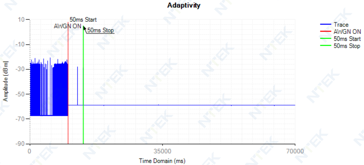
Control Signal NVNT 802.11ac80 5210MHz AWGN
