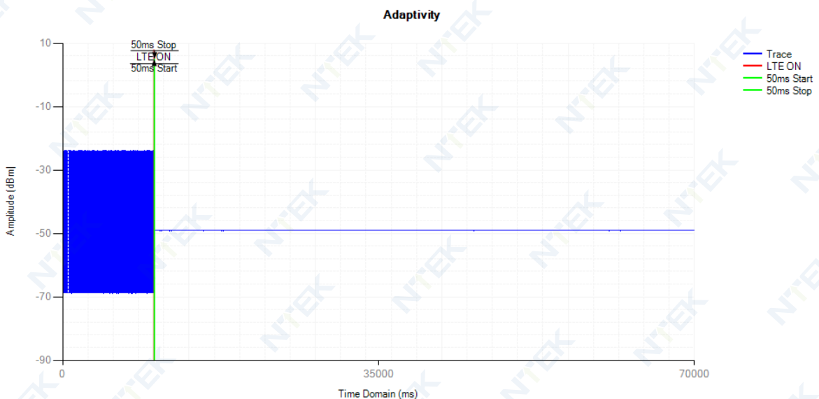
Control Signal NVNT 802.11n(HT40) 5190MHz LTE
