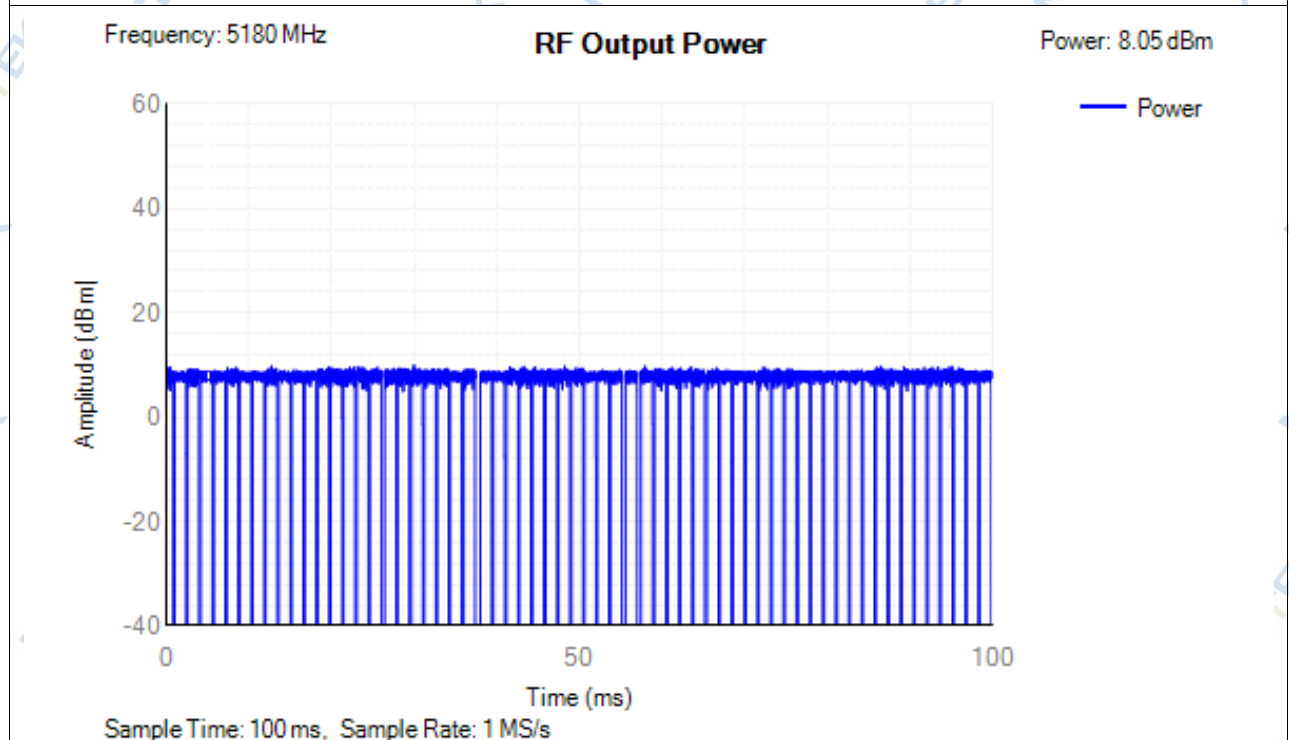
Power NVNT a 5180MHz Ant1
