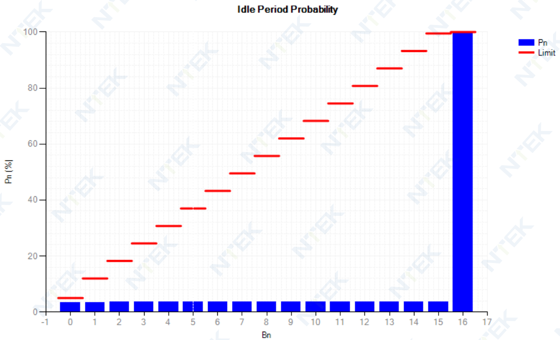
Idle Period Probability NVNT 802.11a 5320MHz
