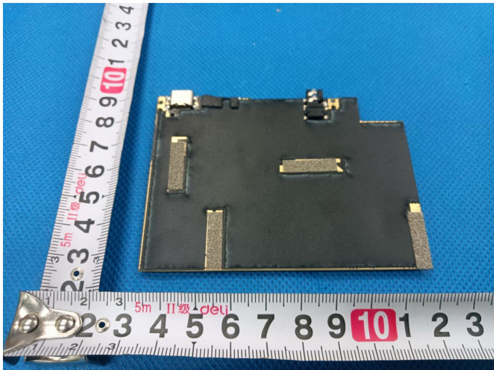
Photo 8 PCB bottom view
