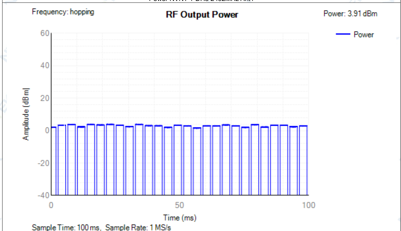
Power NVNT 1-DH5 2402MHz Ant1
