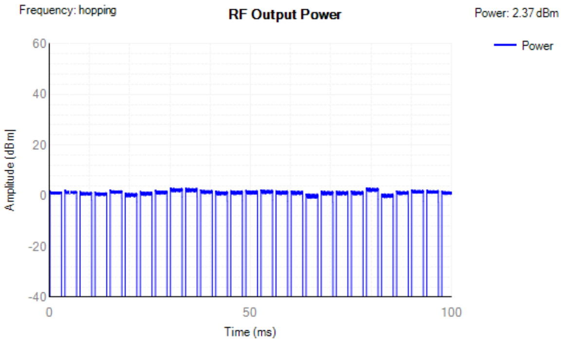
Power NVNT 3-DH5 2402MHz Ant1
