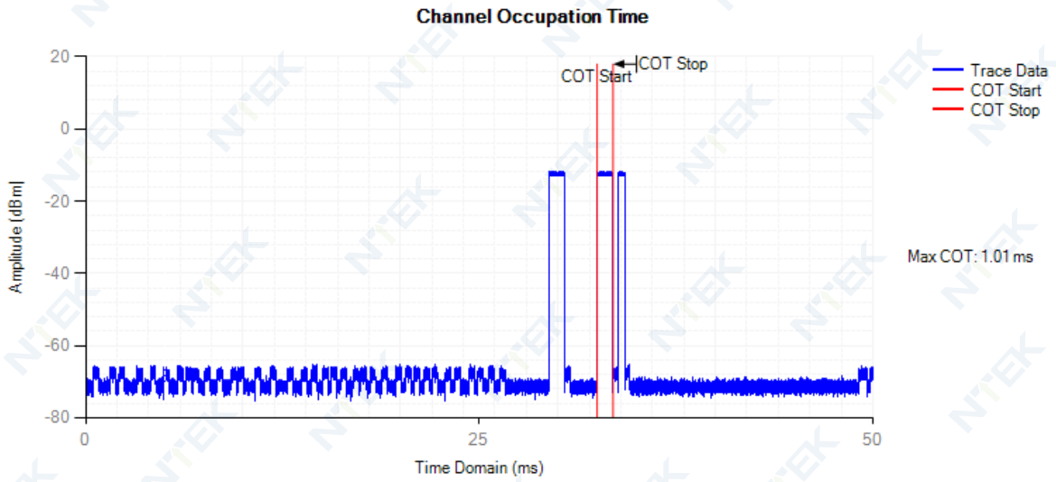
COT NVNT 802.11ax20 2412MHz
