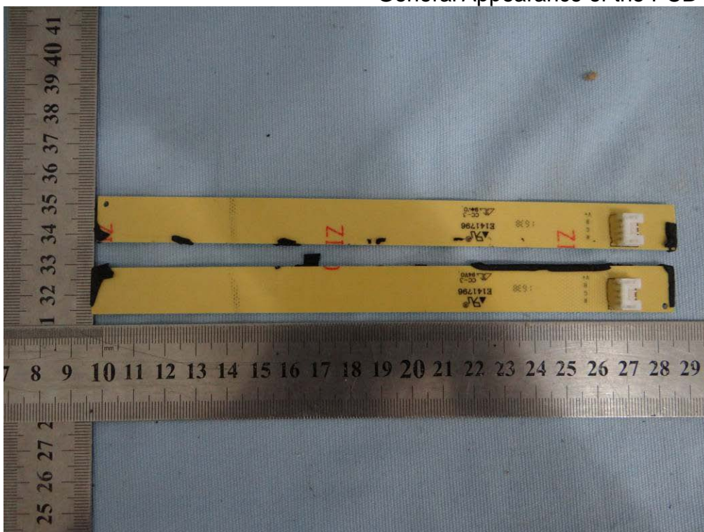
Figure 22 General Appearance of the PCB
