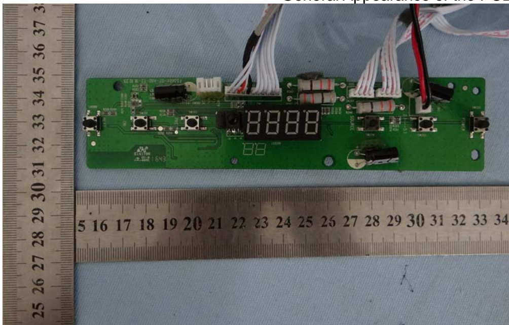
Figure 23 General Appearance of the PCB
