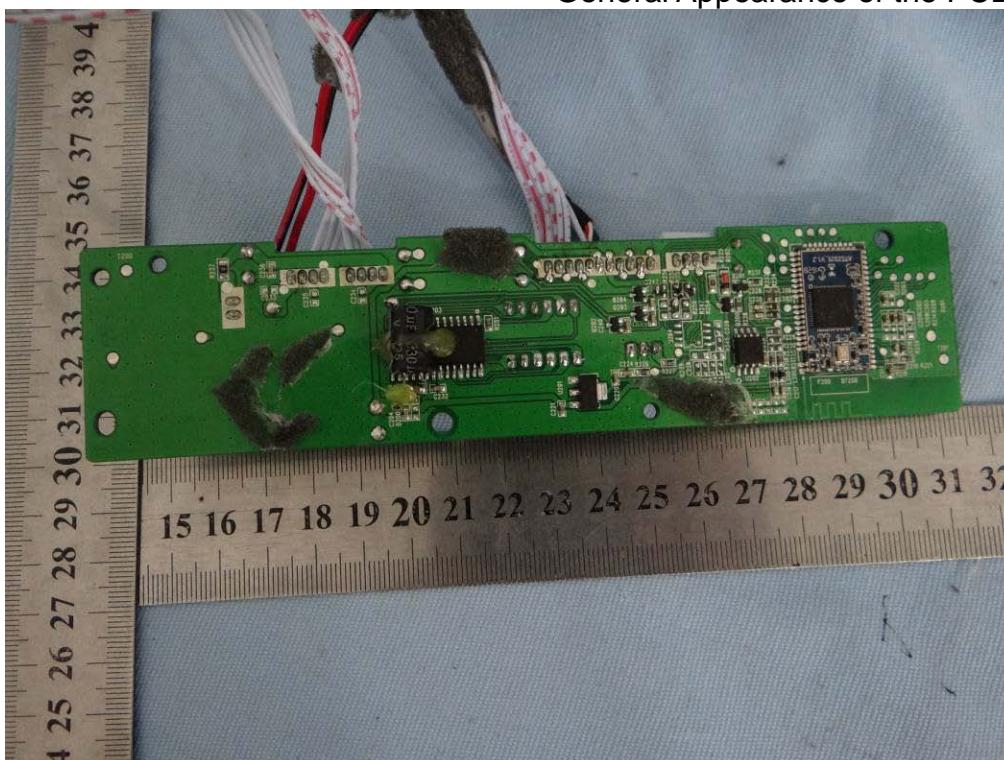
Figure 24 General Appearance of the PCB
