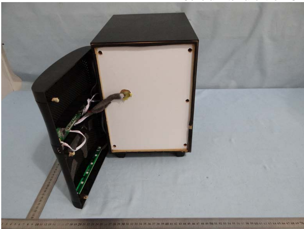
Figure 16 General Internal of the E.U.T.
